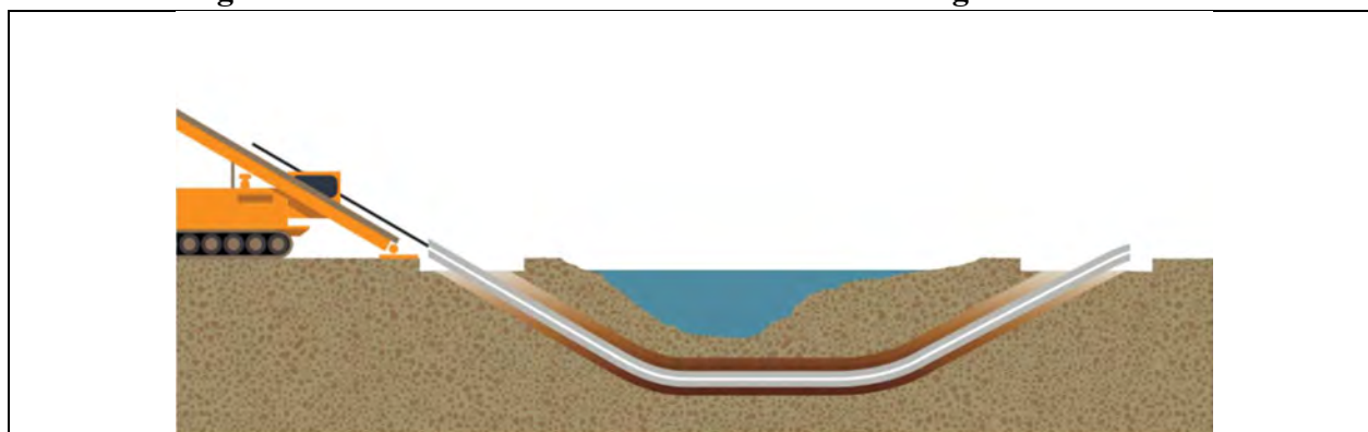
Figure 8. Schematic of horizontal directional drilling under a river 100
