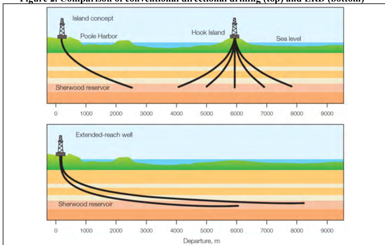
Figure 2. Comparison of conventional directional drilling (top) and ERD (bottom) 48
