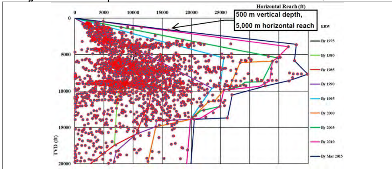
Figure 4. Vertical depth and horizontal reach of ERD wells, worldwide, as of 2015 53
